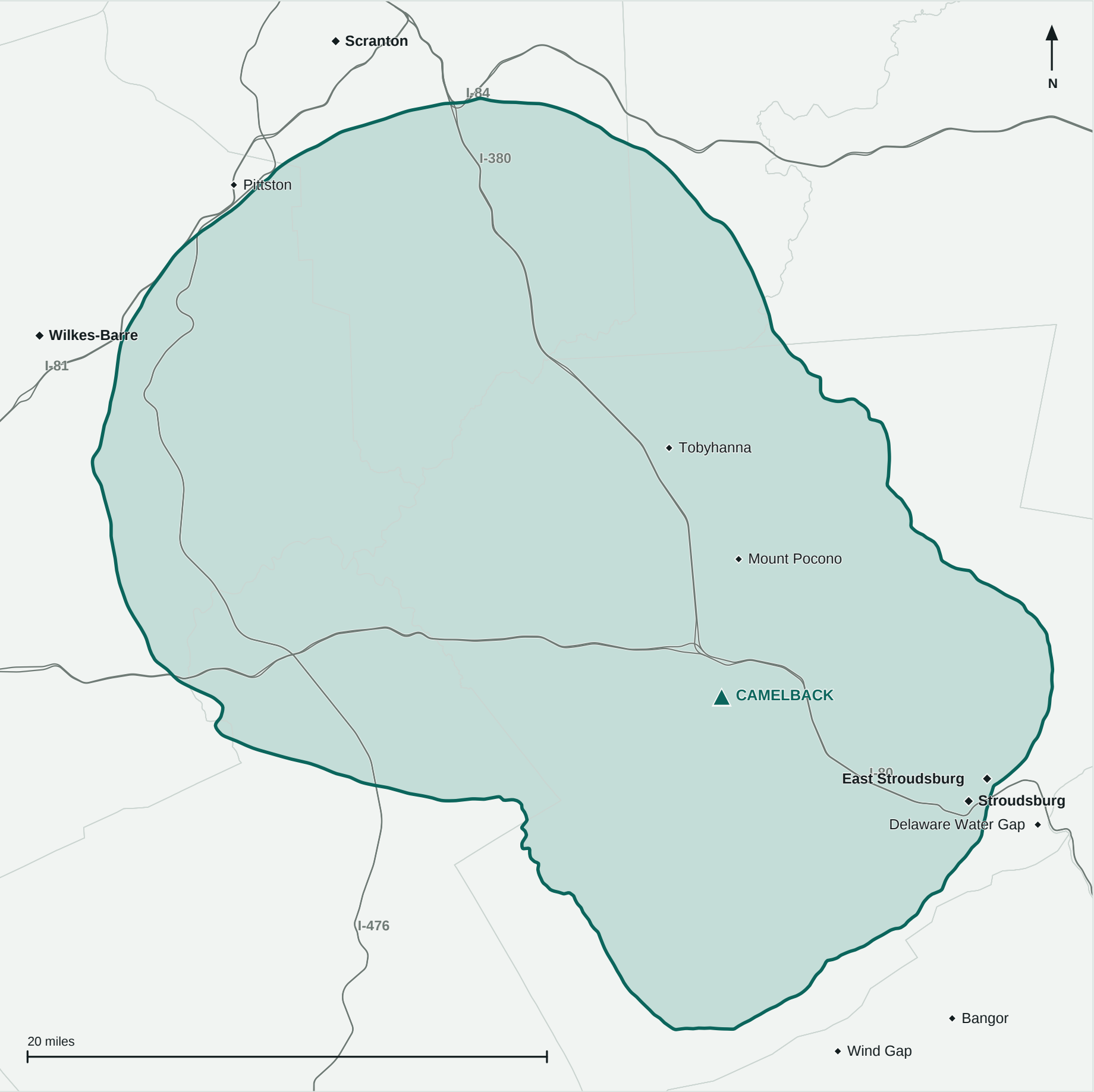
50.2 dBu service contour
